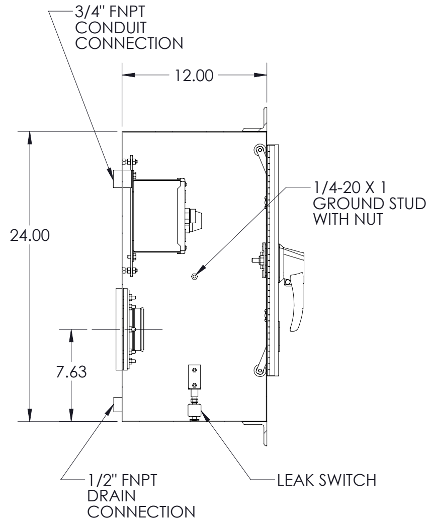
SIDE VIEW/SECTION A-A
